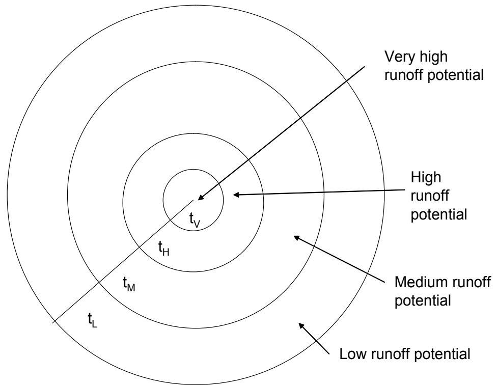
Figure 1. Assumed Spatial Distribution of Soil Phosphorus Runoff Potential.
